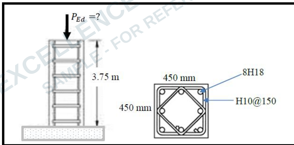
Figure 8: Cross section of the RC column
