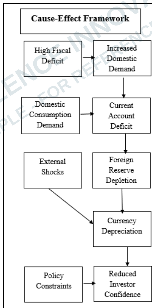
Figure 4.2.1: Cause-Effect Framework
